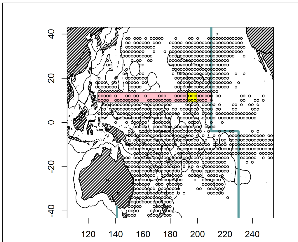
Figure C1. Hotspots of high CPUE (>20 BTH per set) for bigeye thresher shark (BTH). Circles represent locations with at least one observed set gridded to a 2x2 degree resolution. The pink rectangle represents the 9-13°N latitudinal band across the WCPF Convention Area where 83% of the high BTH CPUE sets occurred. The yellow sub-rectangle represents the 193-199°E (161-167°W) longitudinal band where 58% of the high BTH CPUE sets occurred.
