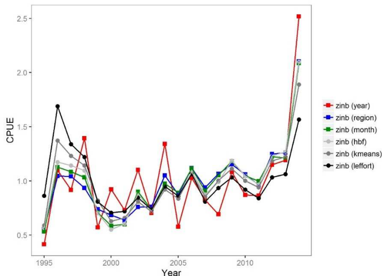
Figure H1: Comparison of annual CPUE indices for BTH in the Calibration Area, as obtained from ZINB models fitted to US Hawaii observer data 1995–2014, where variables were added to each model sequentially (see Table H1). All indices were normalized by the mean of each series for comparison.
